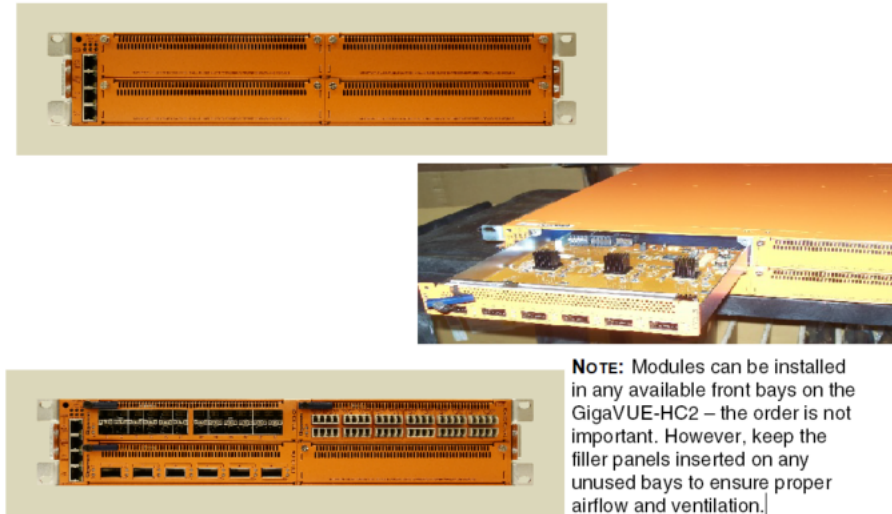
Figure 11 Installing Modules
