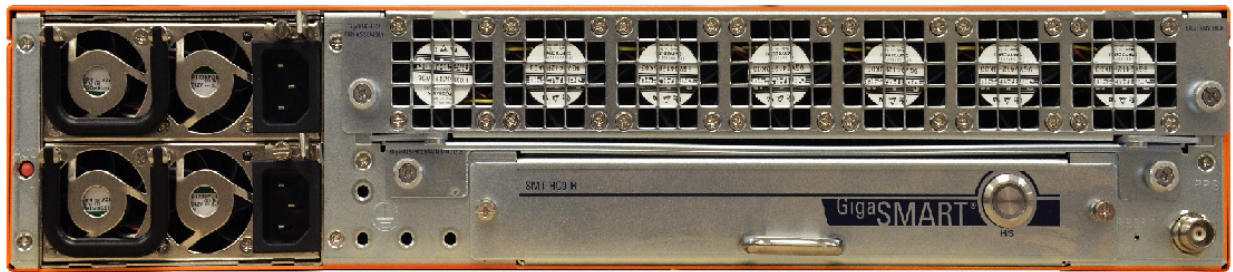
Power module - Three-prong power supply
