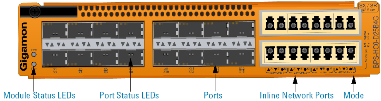
Figure 14 Bypass Combo Module BPS-HC0-D25B4G
