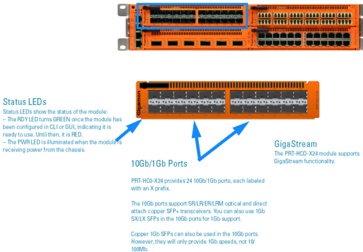
Figure 4 PRT-HC0-X24 Module
