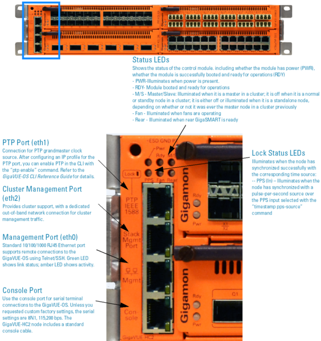
Figure 3 GigaVUE-HC2 Management Ports
