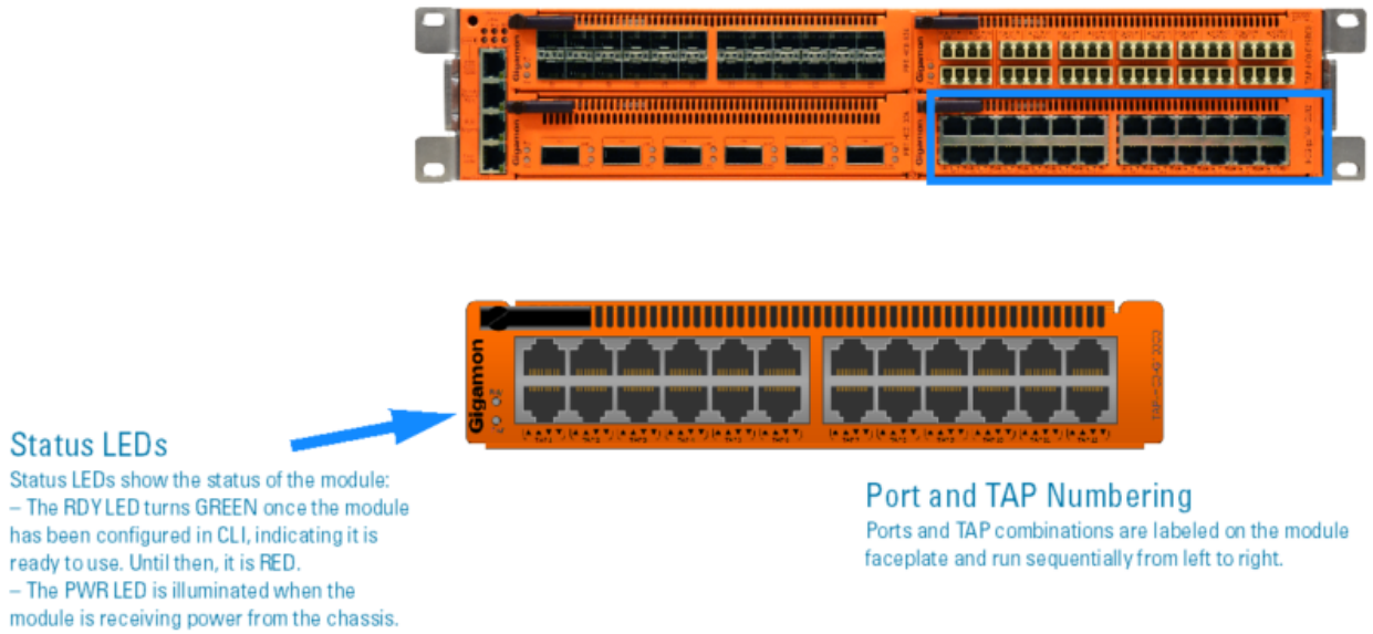
Figure 12 TAP-HC0-G100C0 Module
