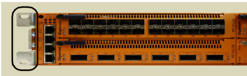
Figure 2 Rack Ears for Front Mount (Reverse Rack Ears for Center Mount)
